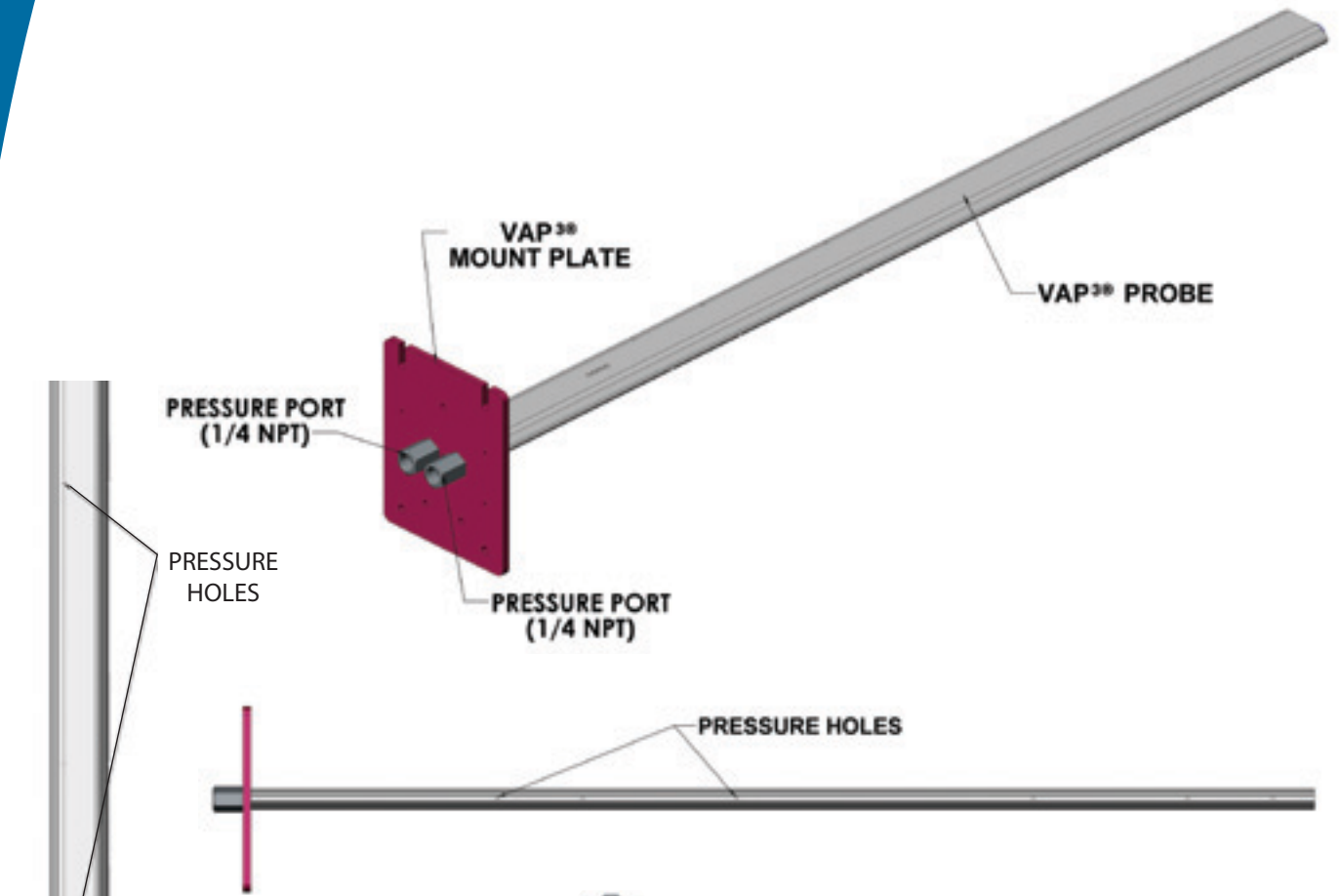
VAP 3 Pitots Circular Duct Installation (front view)
