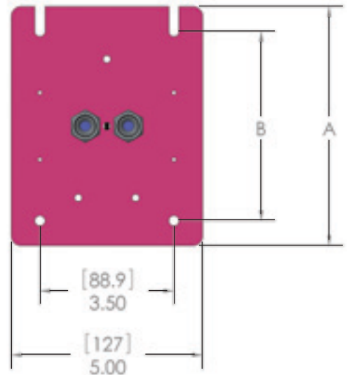
VAP 3 Pitots Circular Duct Installation (isometric view)
