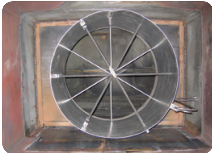
View of the Pitot array within the High Beta®
